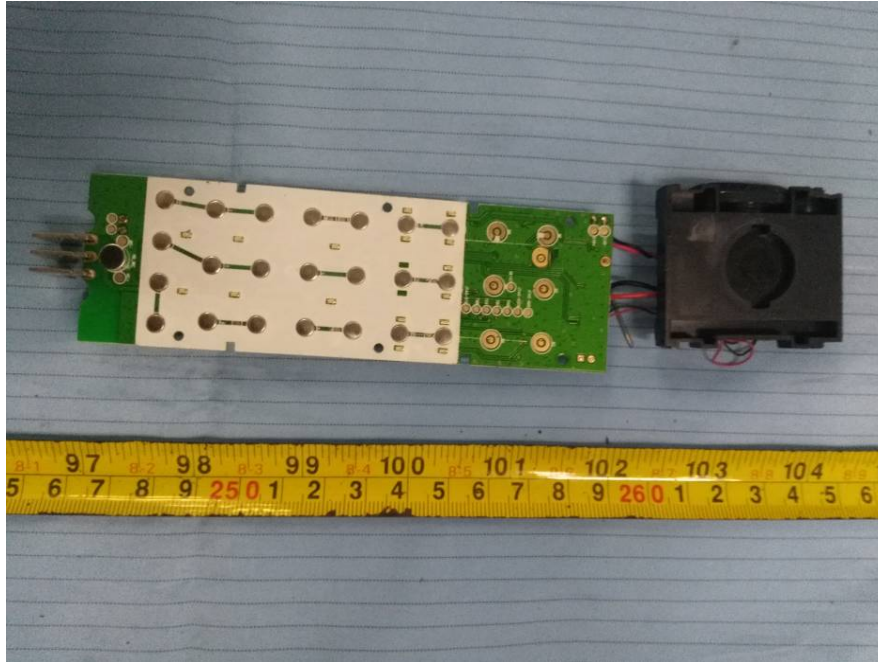
EUT – Main Board Top View (Model: M1035 & M10310 (without memory key))
