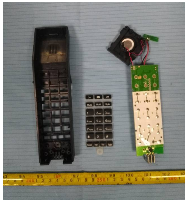
EUT – Cover off View 1 (Model: M1035 & M10310 (without memory key))
