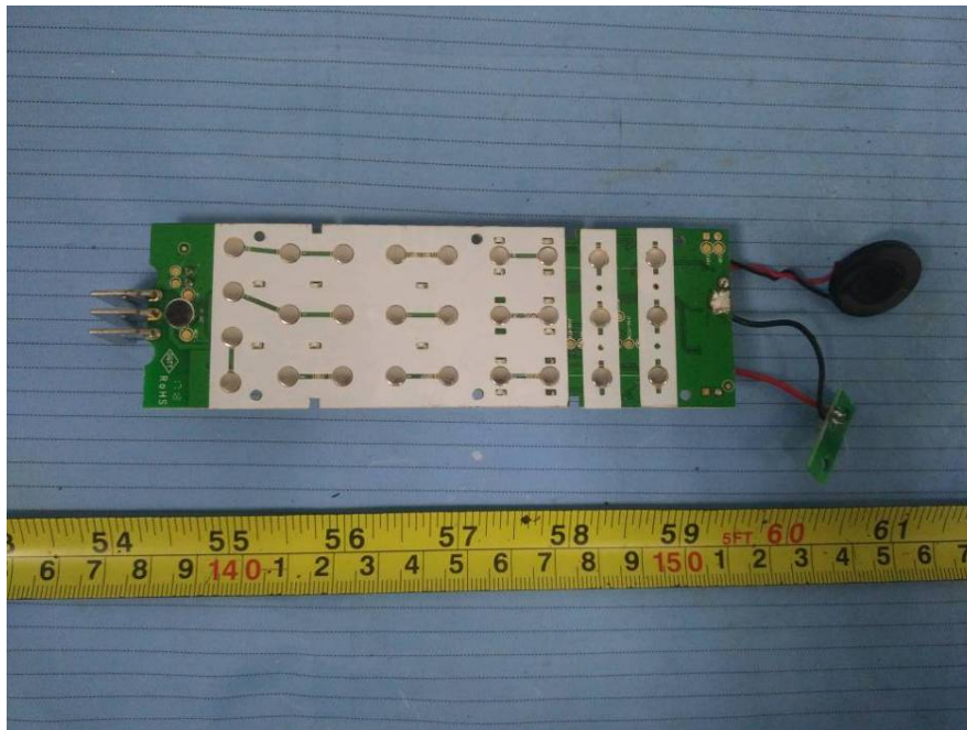
EUT – Main Board Top View (Model: M103106 & M10356 (with 6 memory keys))
