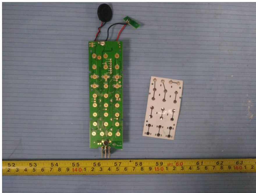
EUT – Main Board Top Shielding off View 2 (Model: M1035 & M10310 (without memory key))
