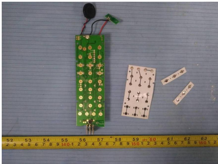
EUT – Main Board Top Shielding off View 2 (Model: M103106 & M10356 (with 6 memory keys))
