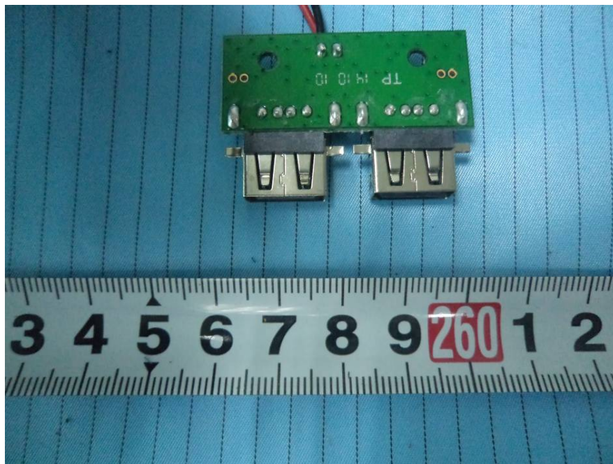
EUT (Base) – Port Board 3 Bottom View
