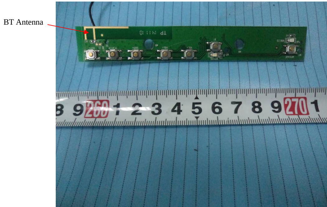
EUT (Base) – Port Board 1 Top View
