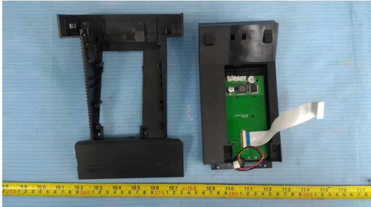
EUT – Cover off View 9
