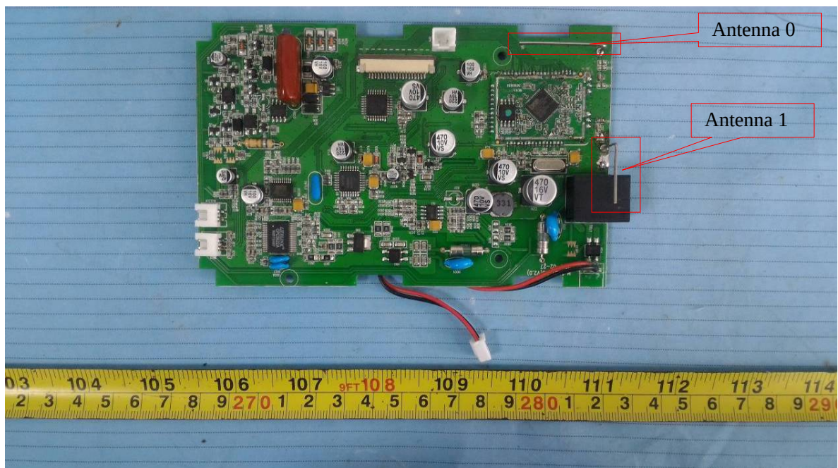
EU –Main Board 1 Top Shielding off View
