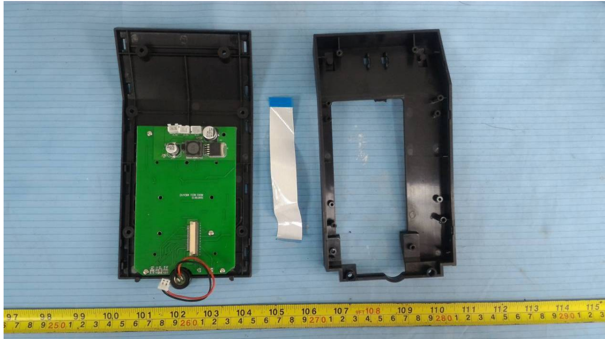
EUT – Cover off View 11
