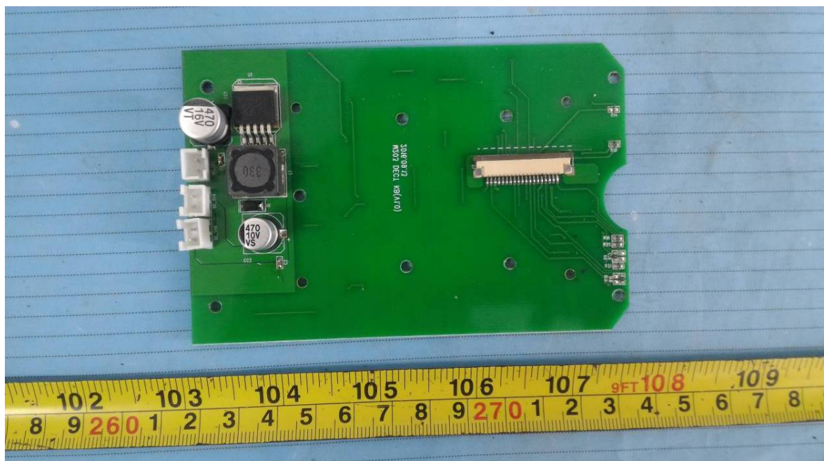
EUT – Main Board 3 Top View
