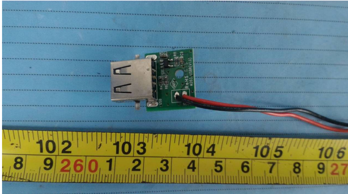
EUT – Right USB Port Top View
