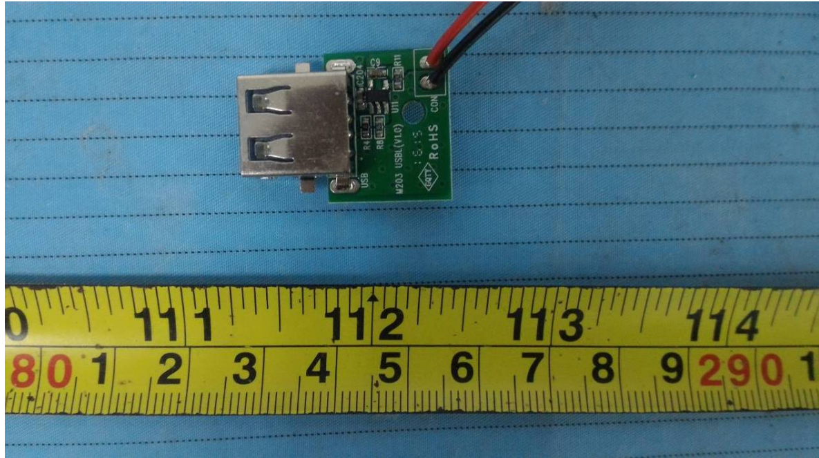
EUT – Left USB Port Top View
