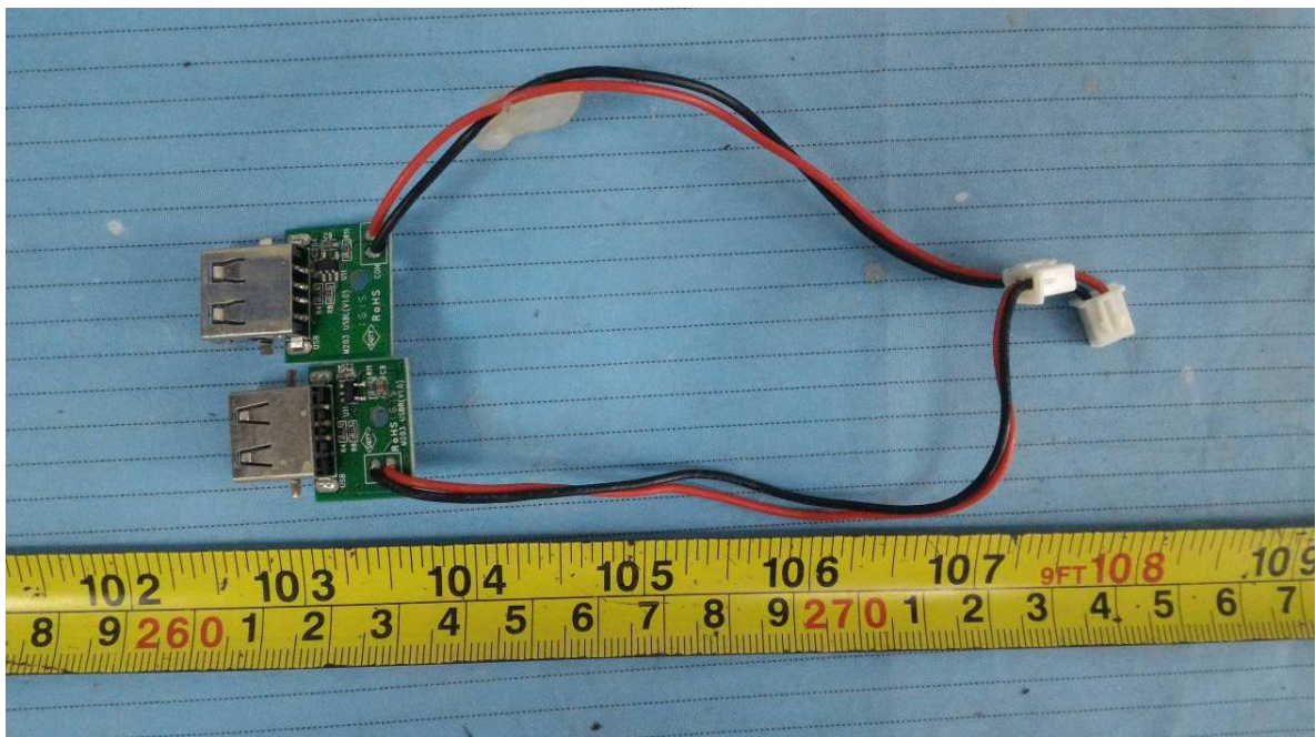
EUT – All USB Port View
