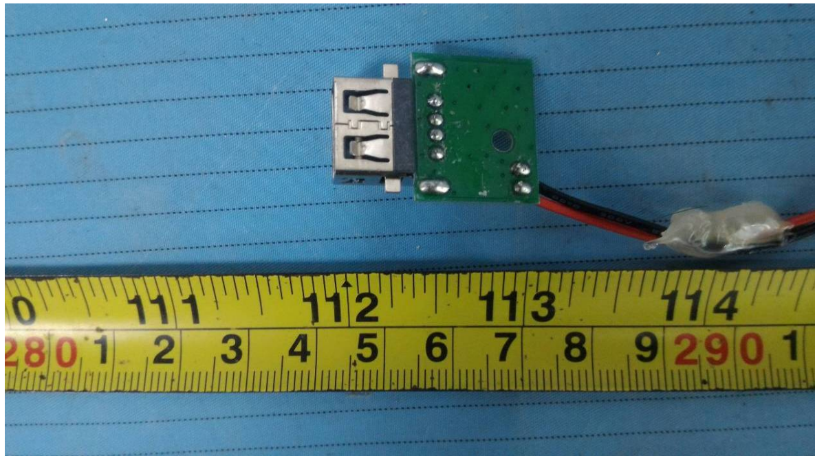
EUT – Left USB Port Bottom View
