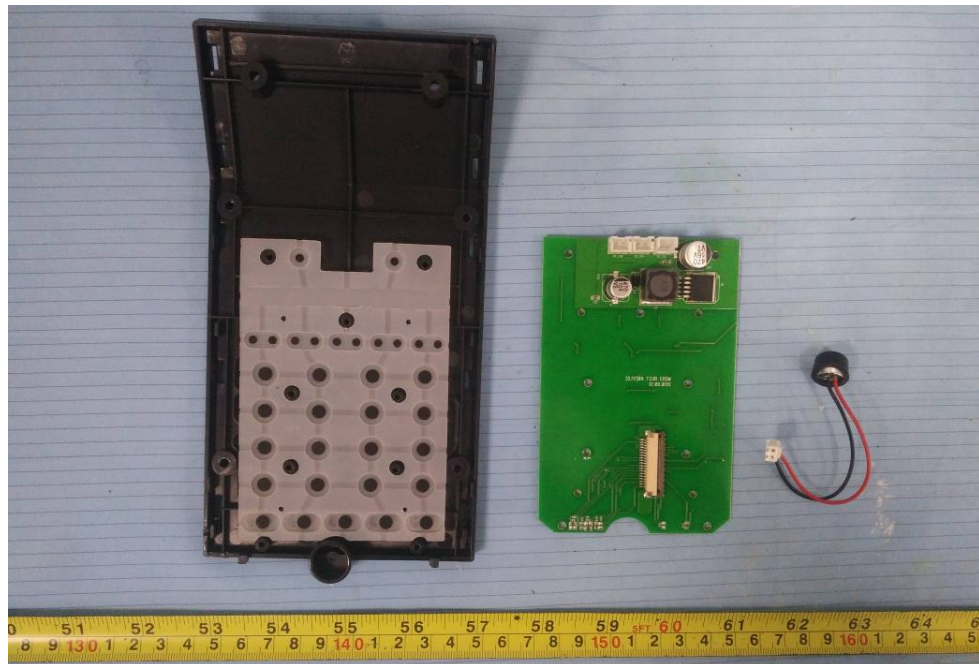
EUT – Cover off View 3(Model: M2035 & M20353 & M20356 (with 5 memory keys))
