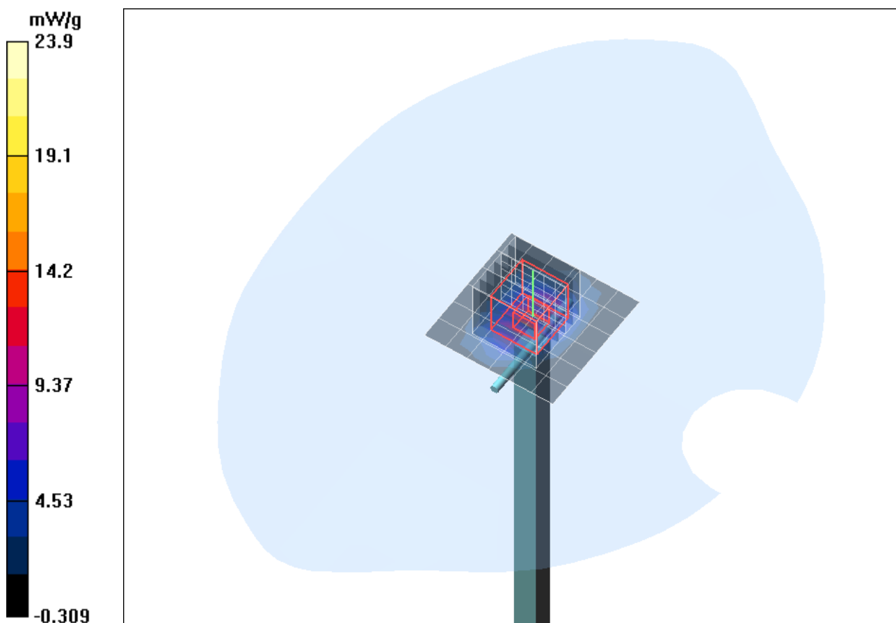
Fig. 9: Validation measurement 2450 MHz Body (May 20, 2011), coarse grid. Ambient Temperature: 21.9° C, Liquid Temperature: 21.6° C.
