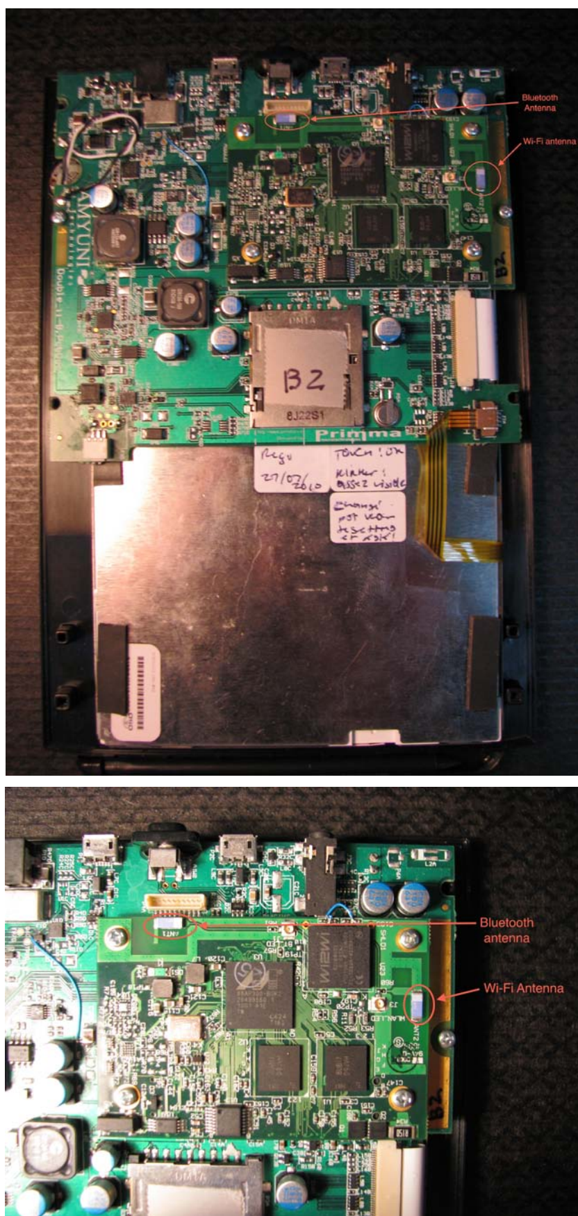
Fig. 13: Picture of the Wi-Fi antenna position.
