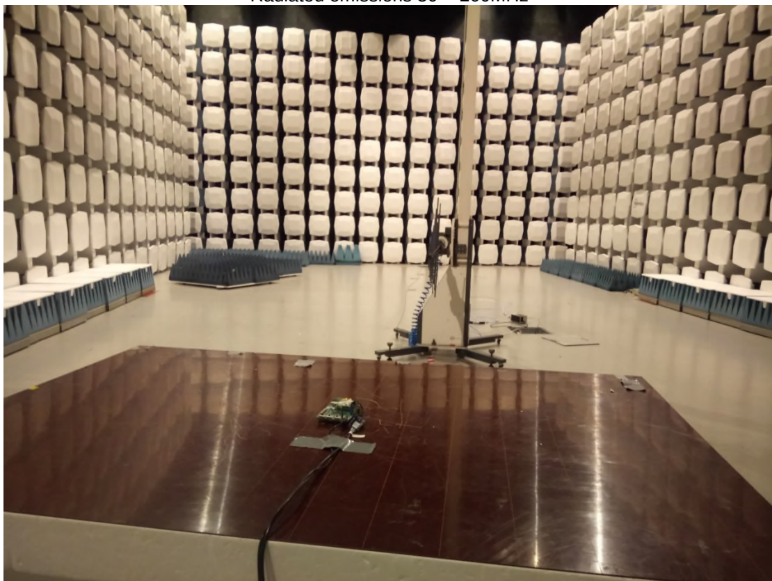
Radiated emissions 200 - 1000MHz
