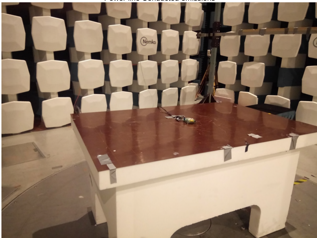
Radiated emissions set-up
