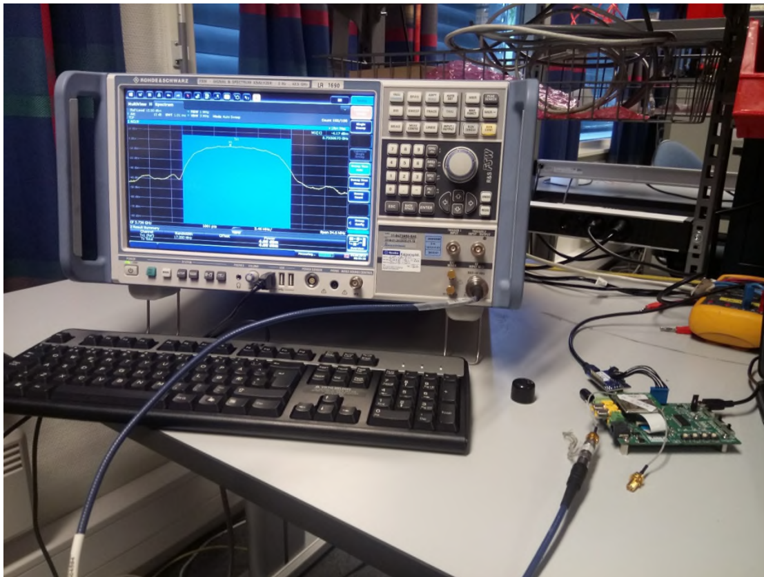
Conducted radio Measurements
