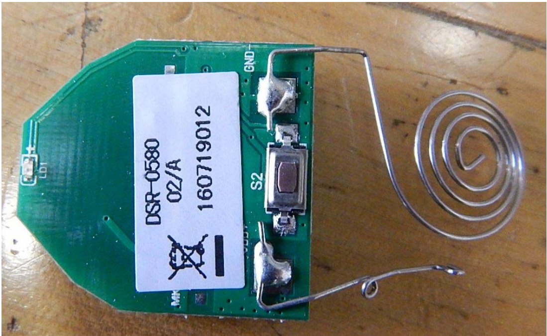
Figure 1-1: Main PCB top view
