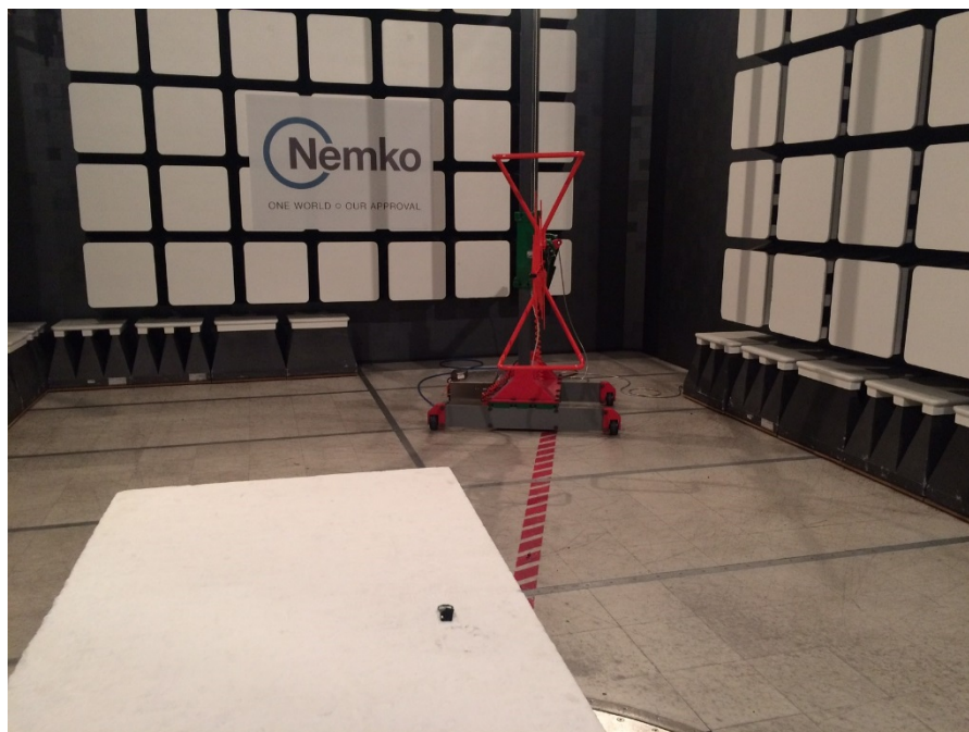
Figure 1-1: Emissions setup photo – 30 to 1000 MHz
