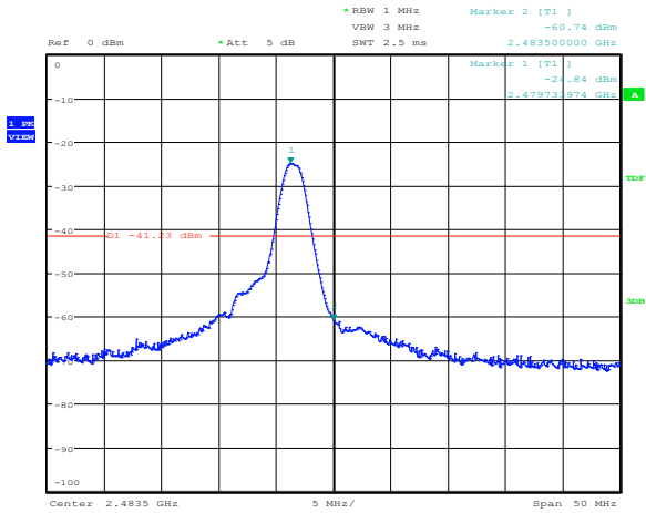
Figure 8.4-8: Conducted spurious emissions outside restricted bands at the upper band edge
