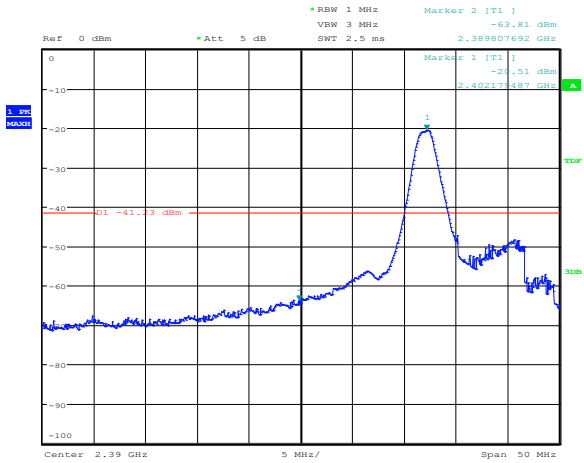
Figure 8.4-7: Conducted spurious emissions outside restricted bands at the lower band edge
