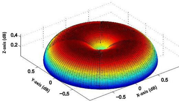
Simulation for radiation pattern of quarter-wave monopole antenna above virtual ground (PCBA)
