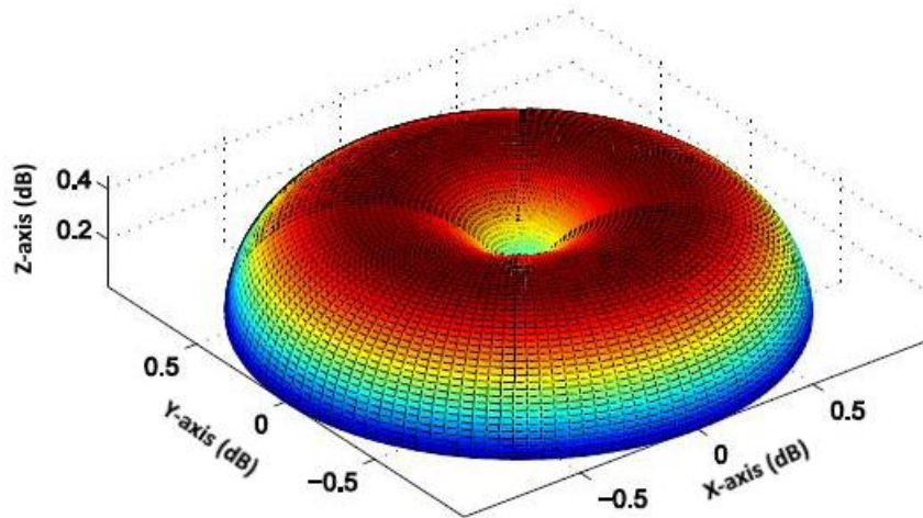
Simulation for radiation pattern of quarter-wave monopole antenna above virtual ground (PCBA)
