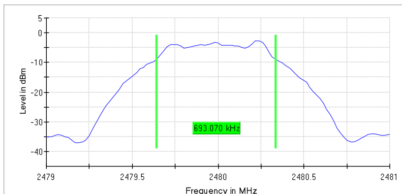
Mode 1 / CH39 (2480MHz)
