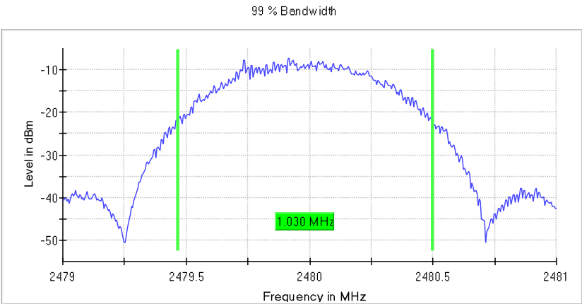
Mode 1 / CH39 (2480 MHz)
