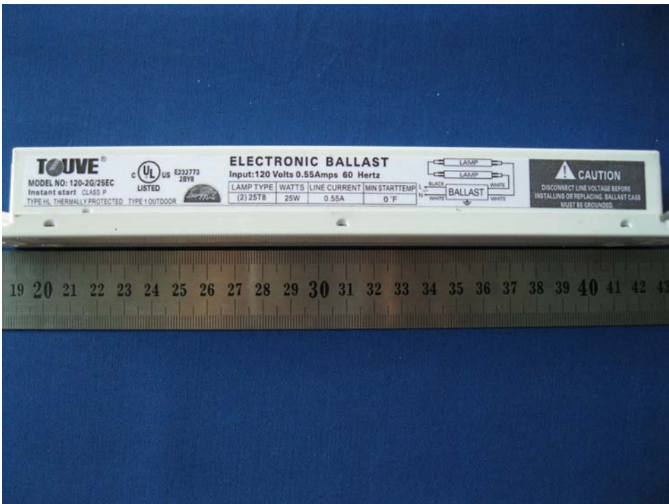
EUT - General View (120-2G/25EC)
