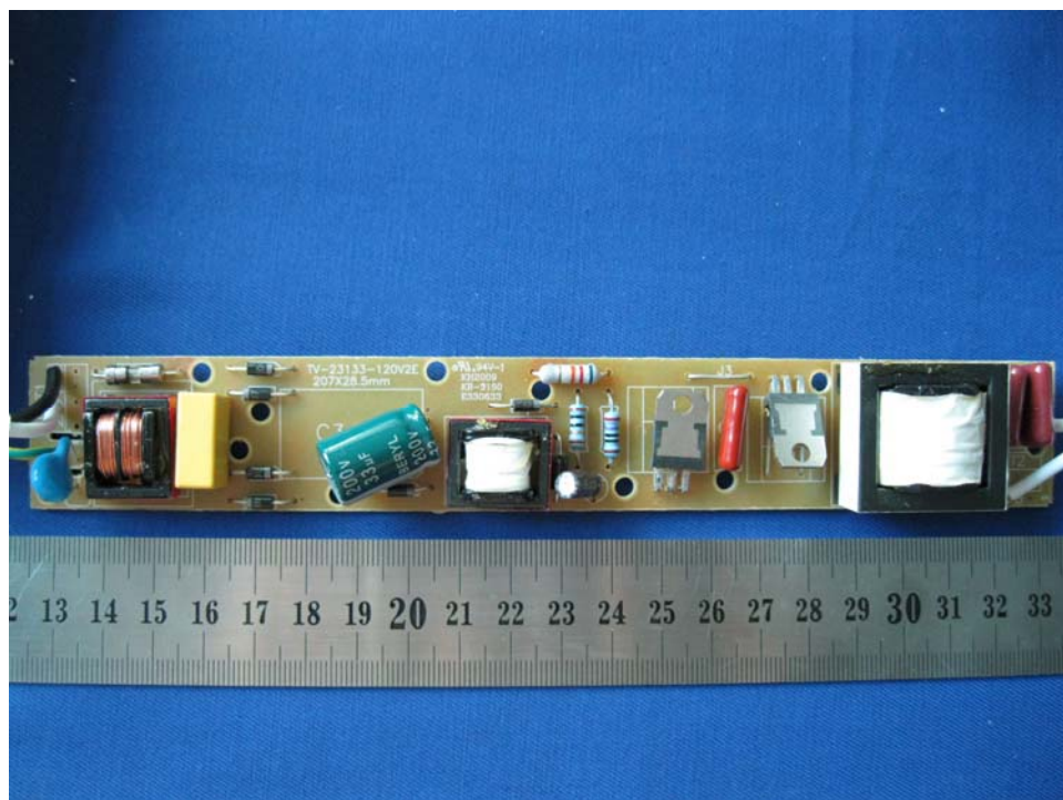
EUT –Components View (120-2G/17EC)
