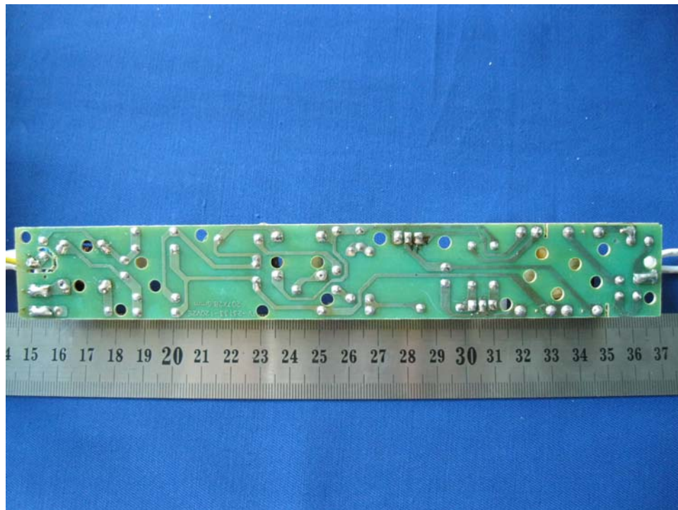
EUT – Uncovered View (120-2G/25EC)
