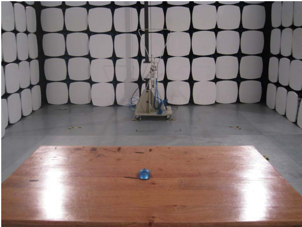
Radiated Measurement Photos (Above 1G)
