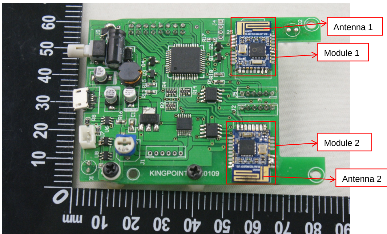
MAIN BOARD TOP VIEW 4
