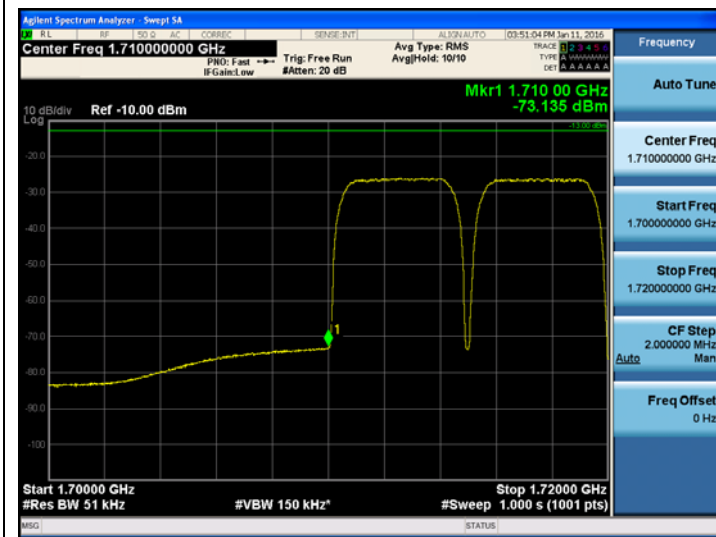
[AWS2100 UMTS Uplink Low]
