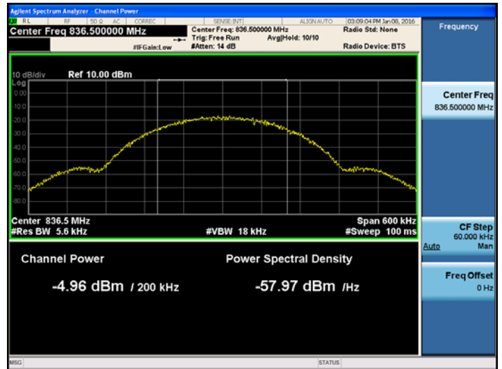
[850Cellular +3dB above the AGC threshold Uplink GSM Mid]
