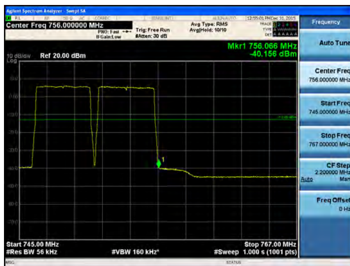
[700 Band LTE 10 MHz Downlink High]
