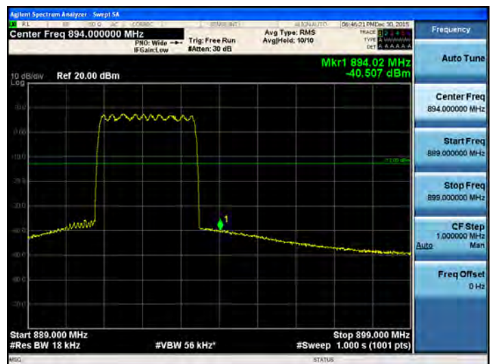
[SMR 800,850 Cellular CDMA Downlink High]
