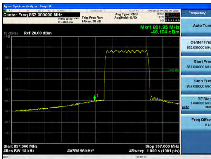
[SMR 800,850 Cellular CDMA Downlink Low]
