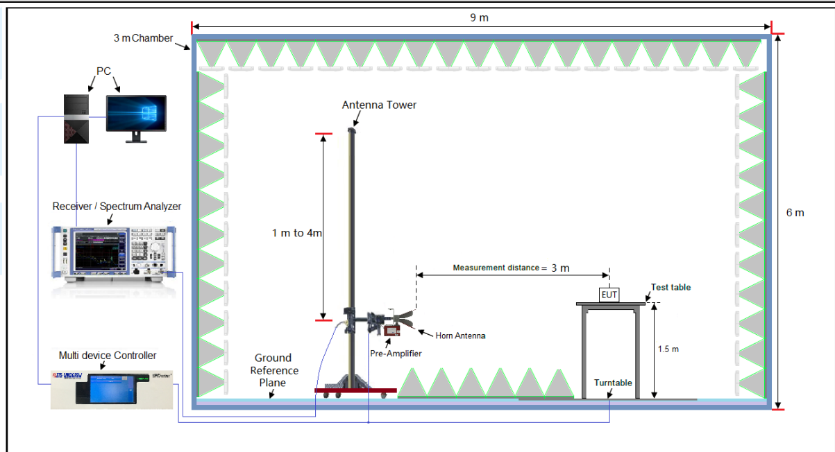
Figure 3. Above 1GHz
