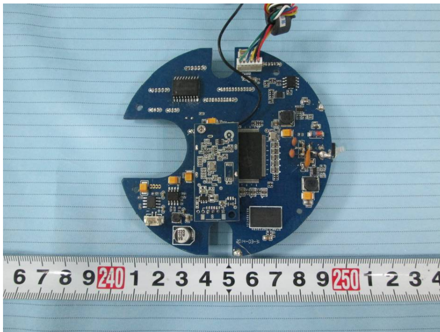
EUT – Main Board Top View (with wifi module)
