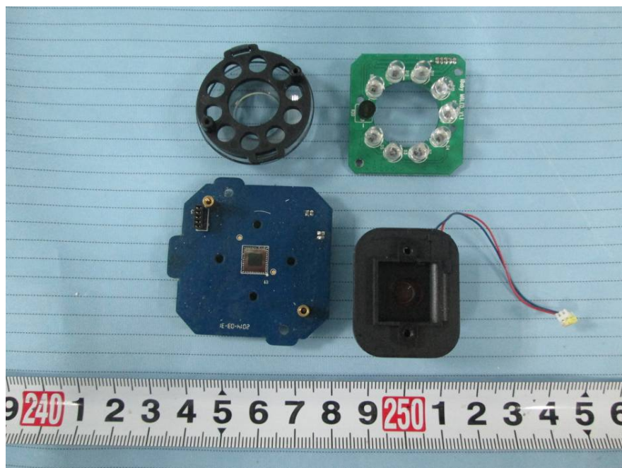
EUT –Sensor Cover off View
