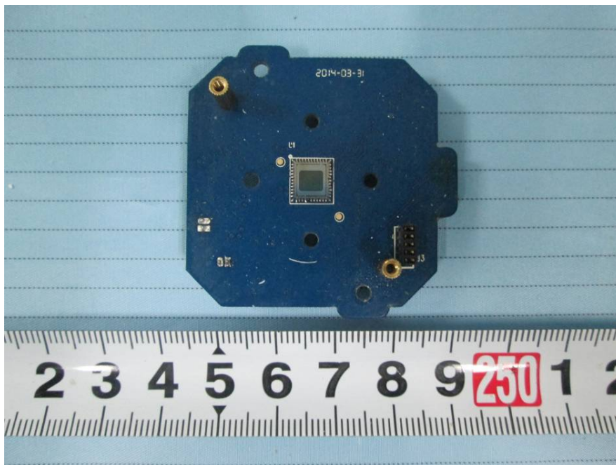
EUT – Sensor Main Board Bottom View
