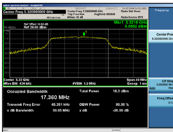
11a CH64 5320
