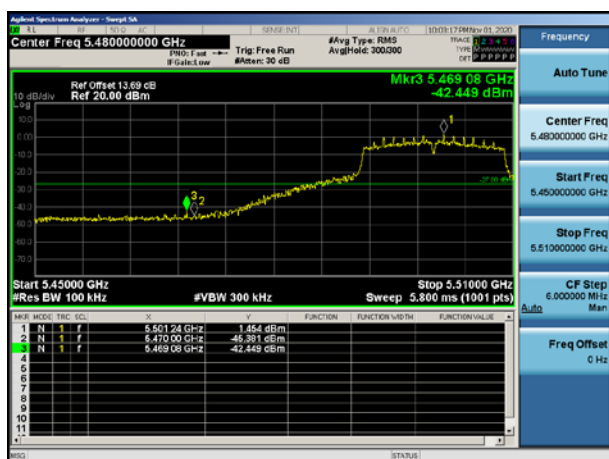
Band edge-Left
