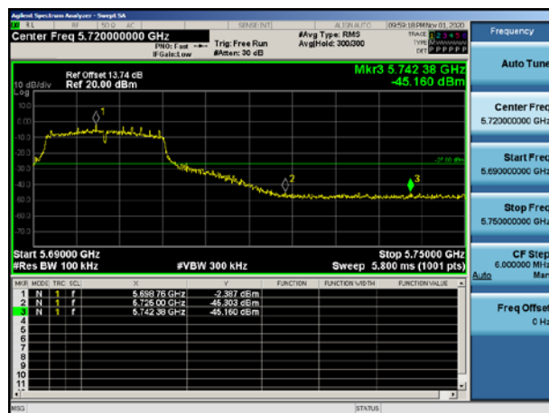
Band edge-Right
