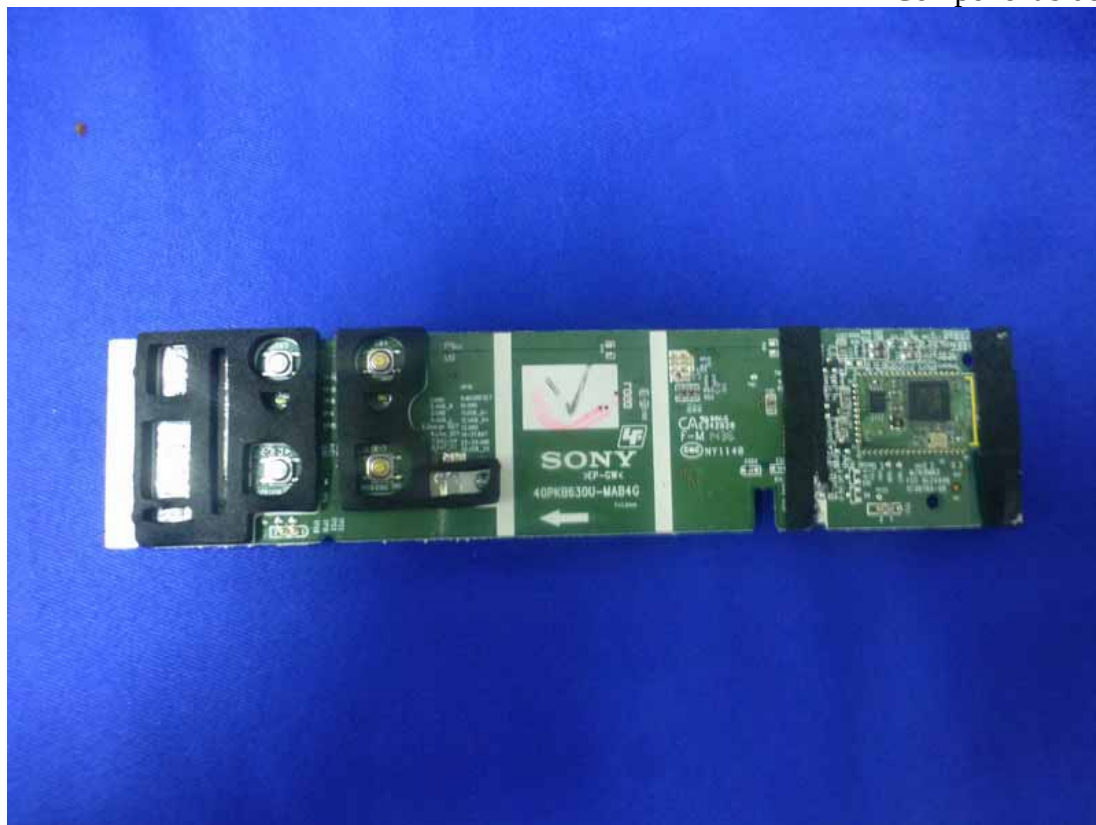
Figure 2 Component side of the PCB
