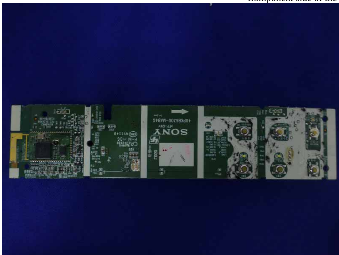
Component side of the Main Board
