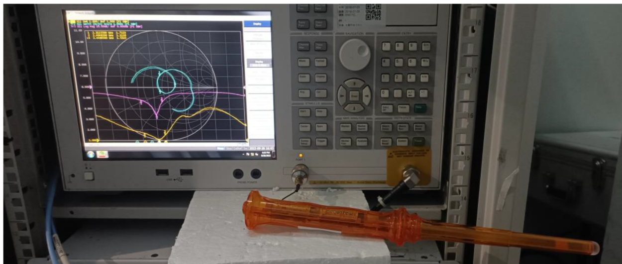
S11 test
