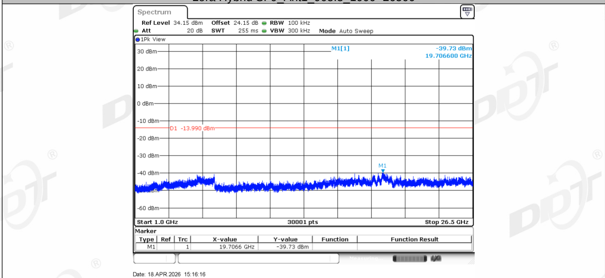
Lora Hybrid SF10_Ant1_903.9_0~Reference
