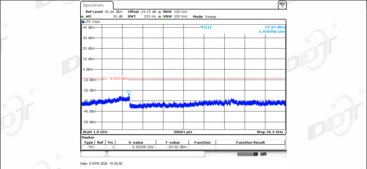
LORA DTS SF7_Ant1_927.5_0~Reference
