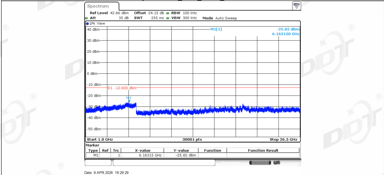
Lora Hybrid SF10_Ant1_904.5_0~Reference
