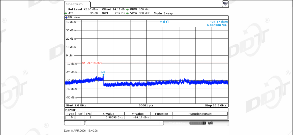
LORA DTS SF8_Ant1_904.6_0~Reference
