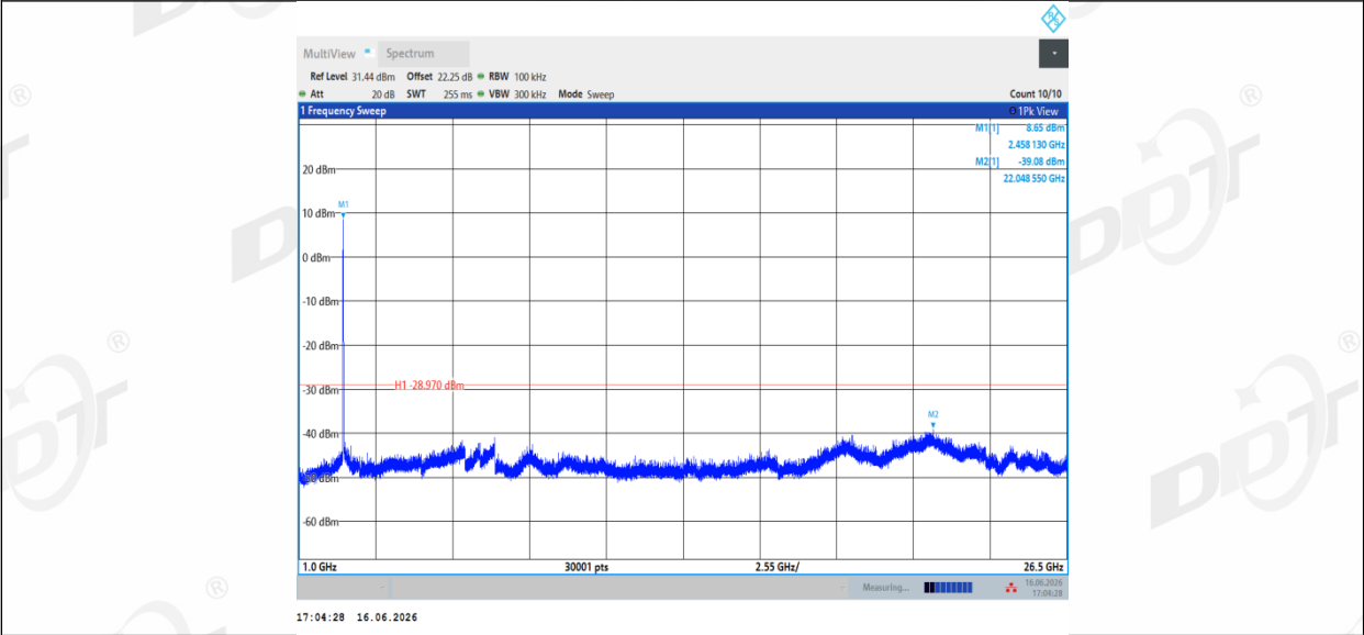
11AX20SISO_Ant1_2462_1000~26500
