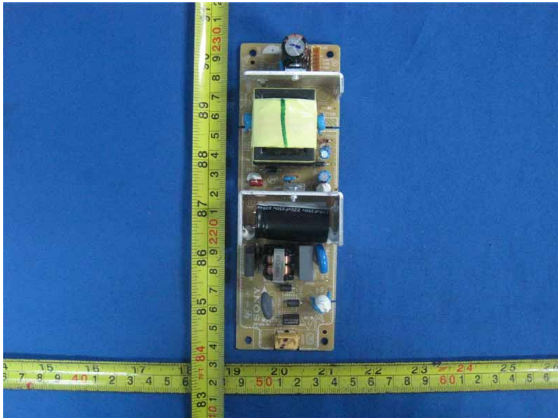
Figure 13 Frontside of the Power Board
