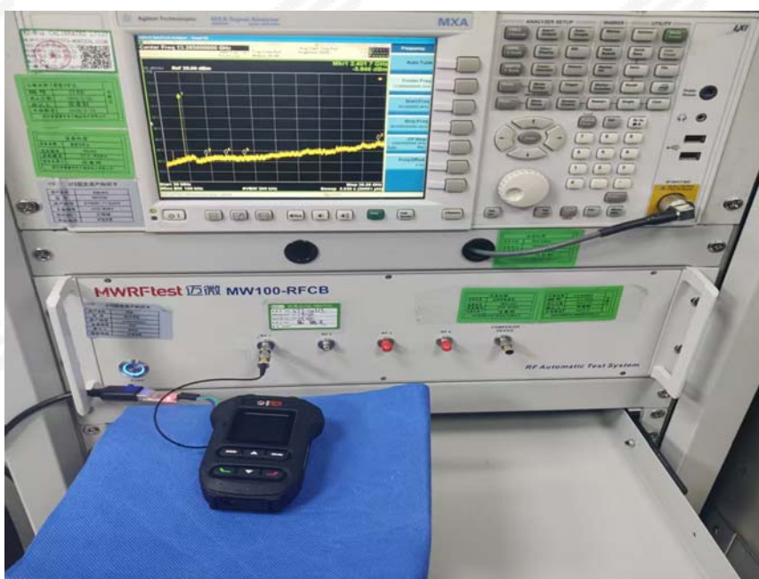
RF Conduction
