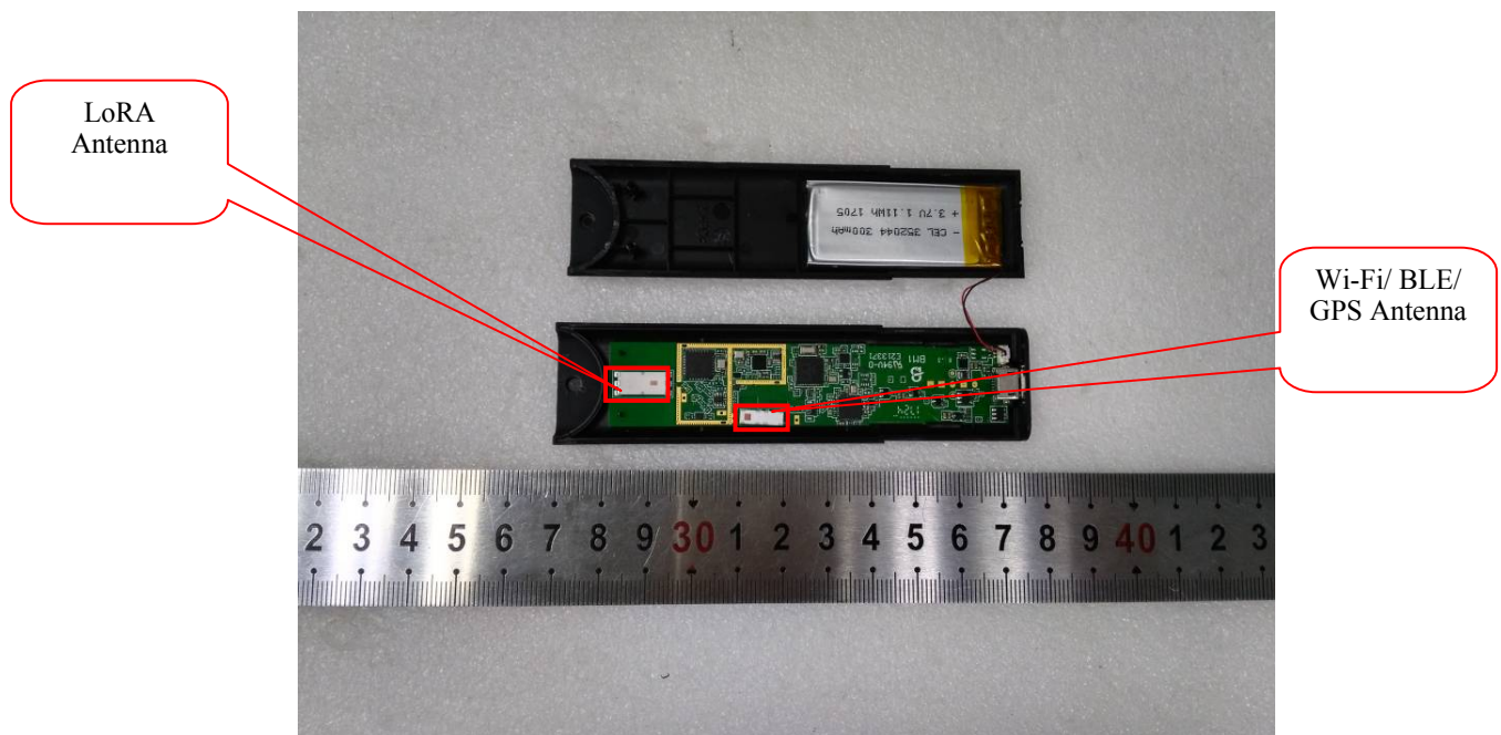
EUT – Cover off View 2
