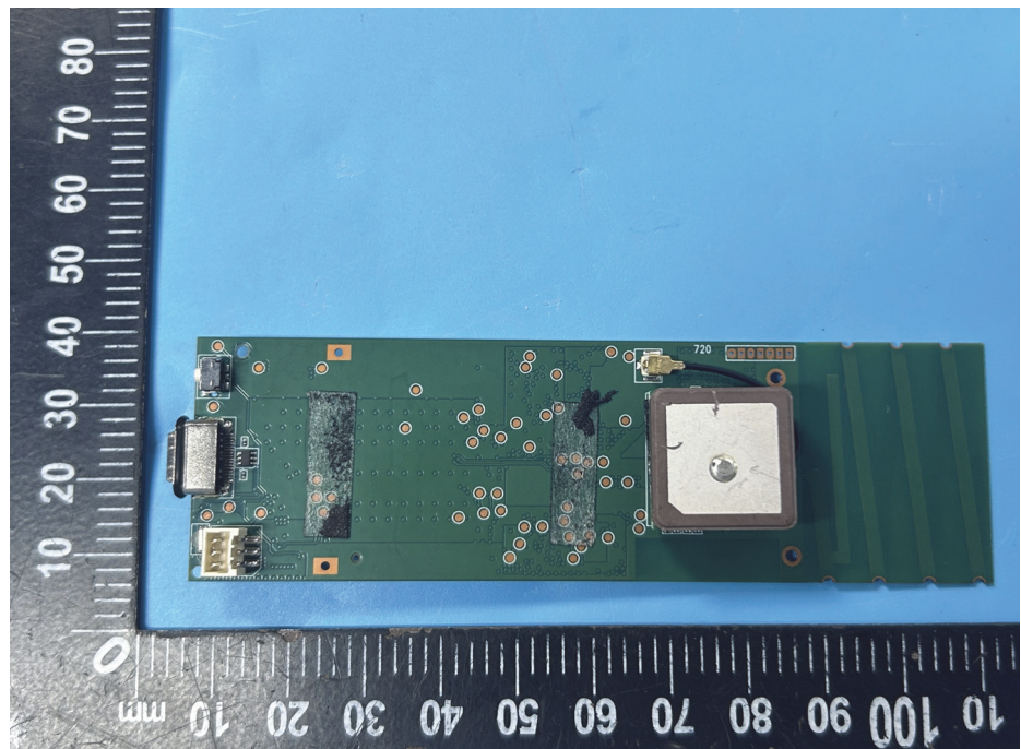
Solder Board-Component View 1
