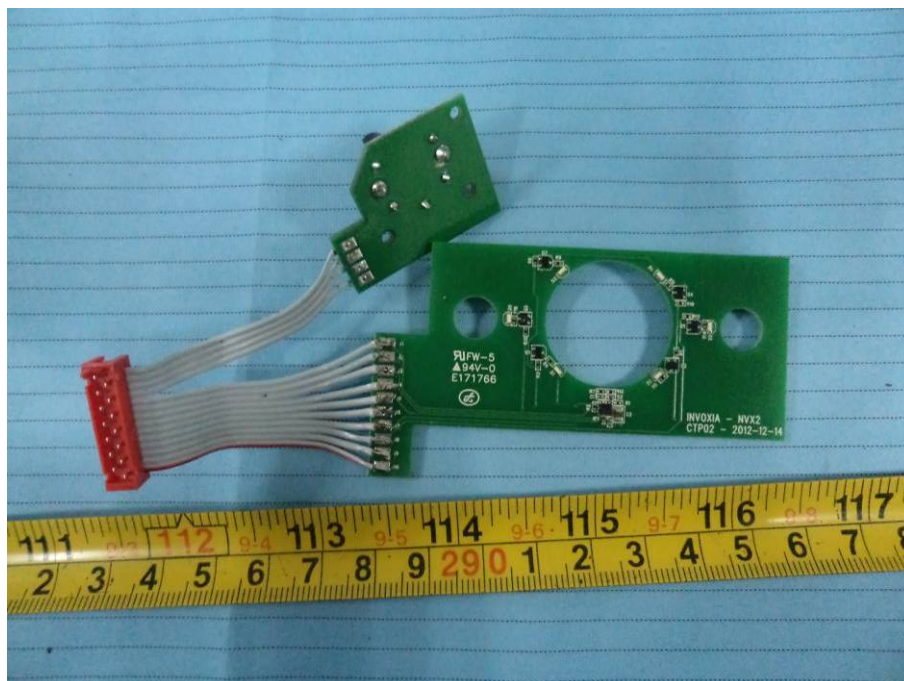
EUT – Loudness Board Bottom View
