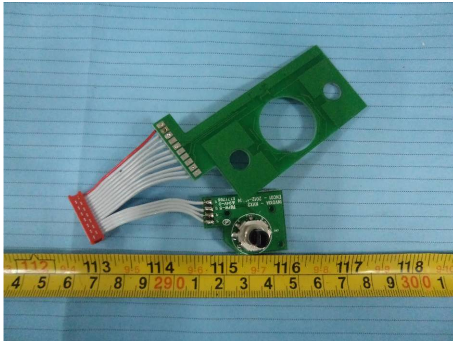
EUT – Loudness Board Top View
