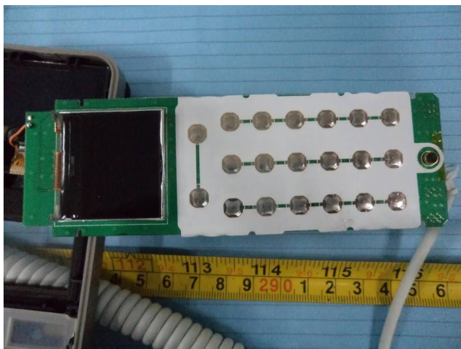
EUT – Microphone Board Top View
