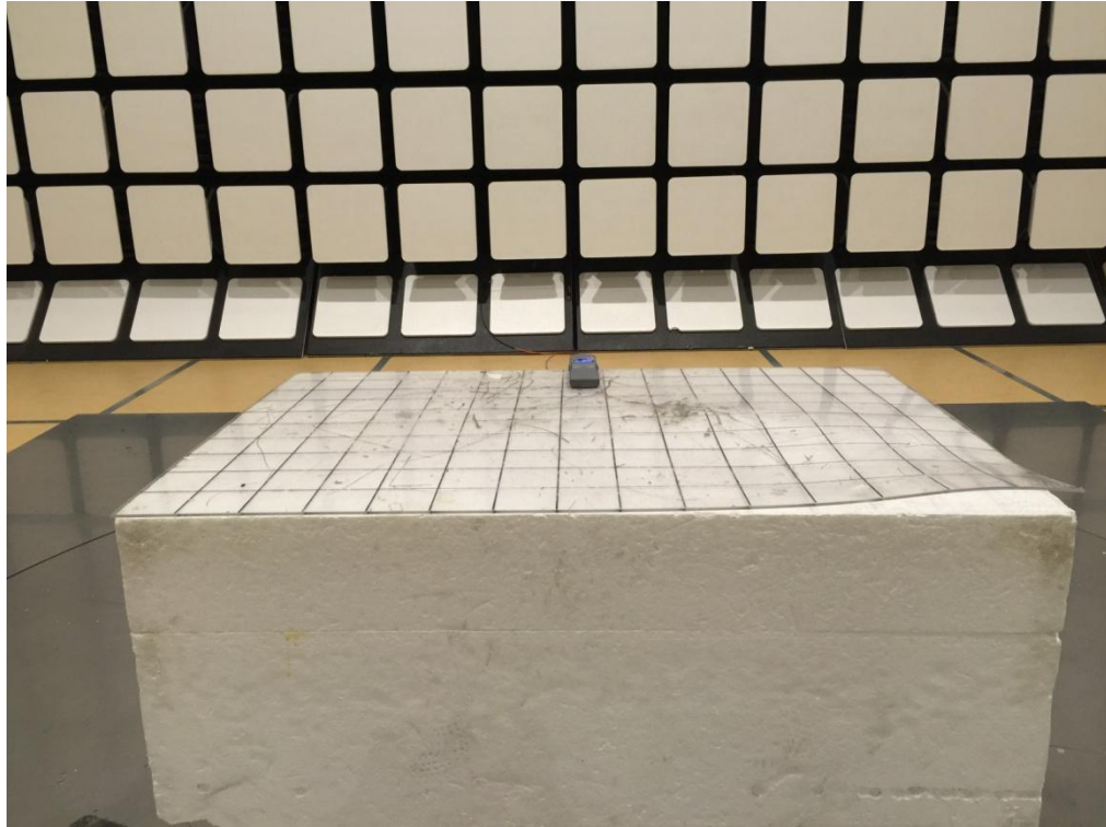
Radiated Emission (Fundamental) Test Setup (Front View)
