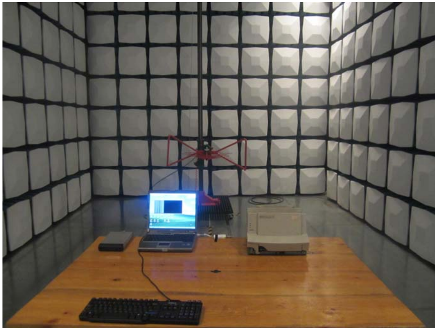
Radiated Emission blew 1 GHz - Rear View
