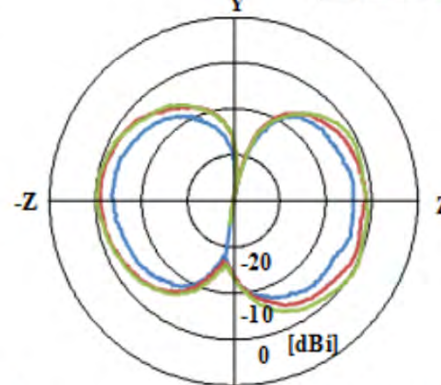
Horizontal-YZ
