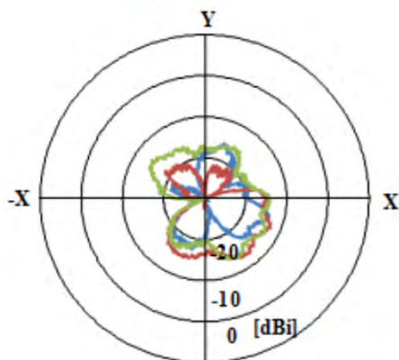
Vertical-XY
