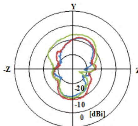
Vertical-YZ
