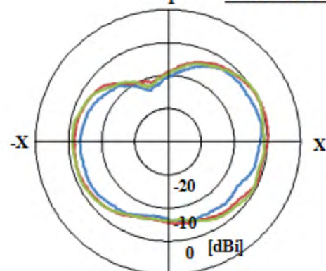
Horizontal-XY
