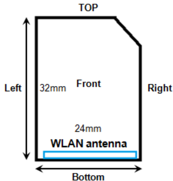
Antenna location
