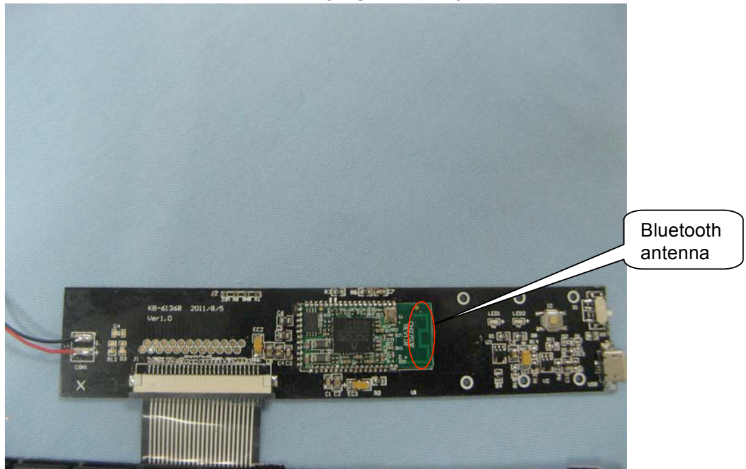
INTERNAL VIEW OF SAMPLE – 3
