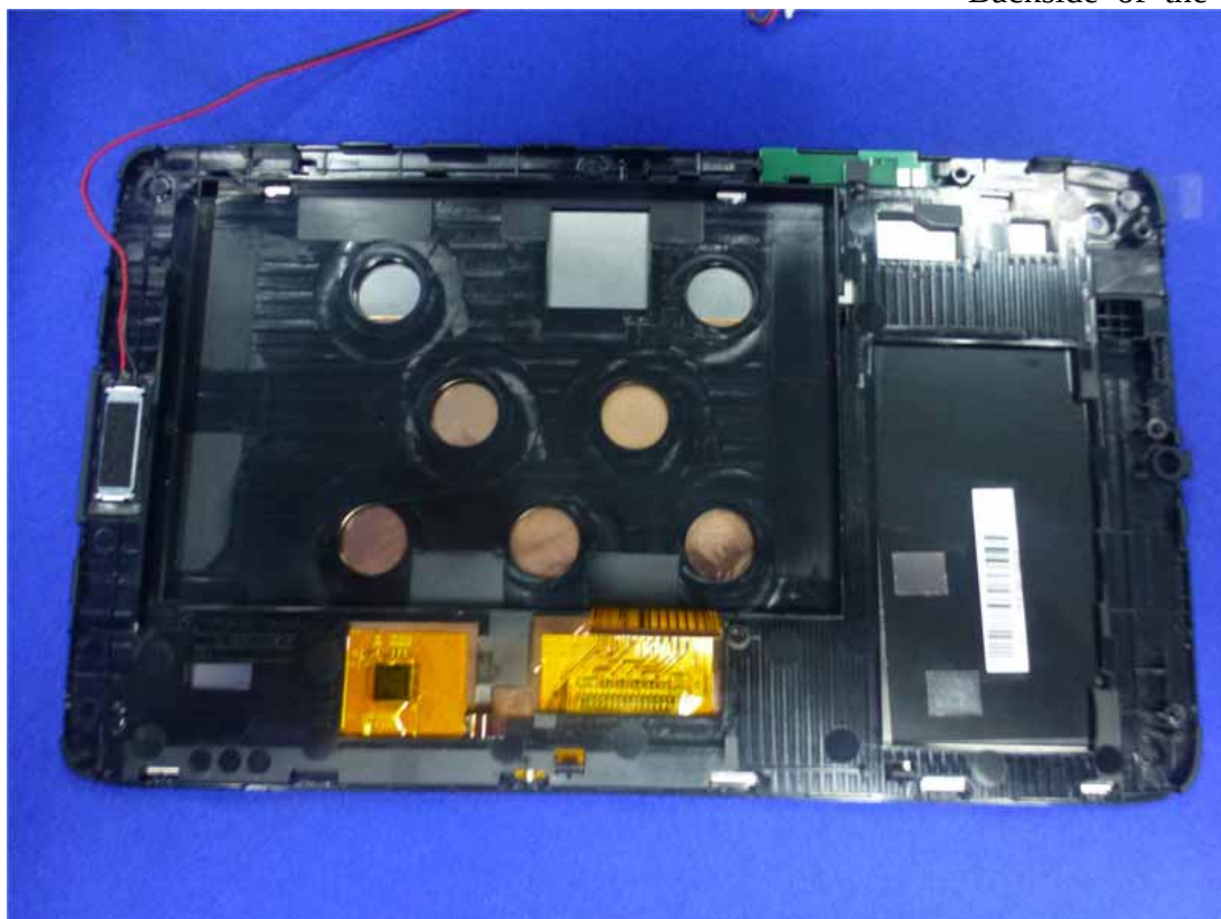
Figure 21 Backside of the LCD Panel
