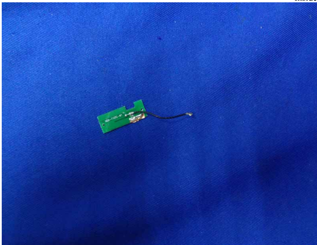
Figure 12 Inside of the EUT
