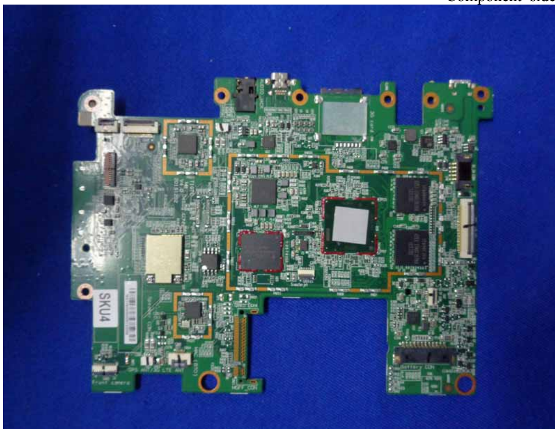
Figure 21 Component side of the PCB
