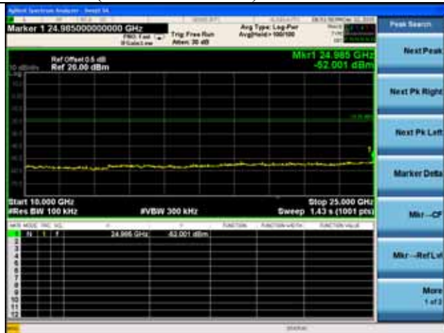
2402MHz(10GHz – 25GHz)
