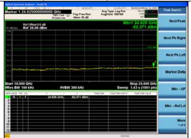
2441MHz(10GHz – 25GHz)
