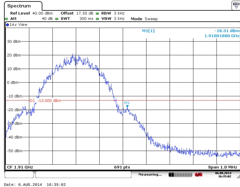
Higher Band Edge Plot on Channel 810 (1909.8 MHz)
