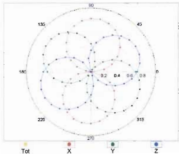
f=600 MHz,TEM
