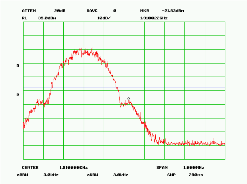
Higher Band Edge Plot – EGPRS1900, Channel 810, High Channel
