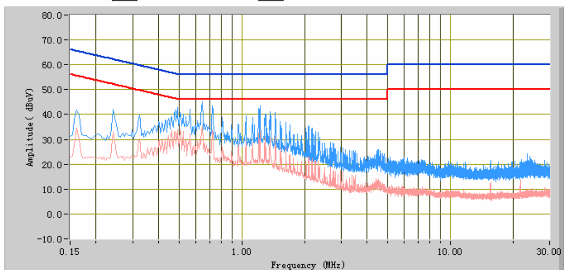
Phase Line Plot at 230Vac, 50Hz
