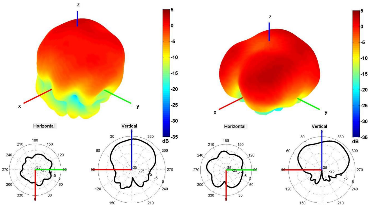
2450 and 5500 MHz Radiation pattern
