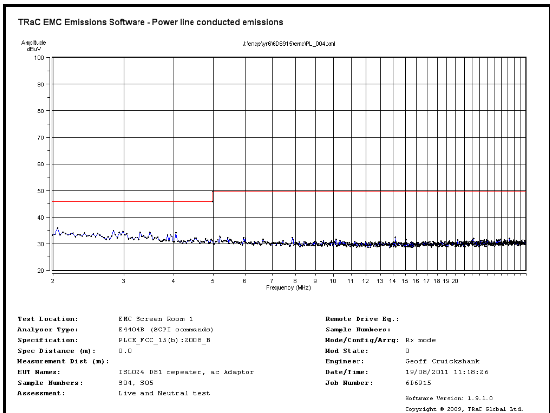
ac Power Line Conducted emissions 2MHz to 30MHz – Rx mode
