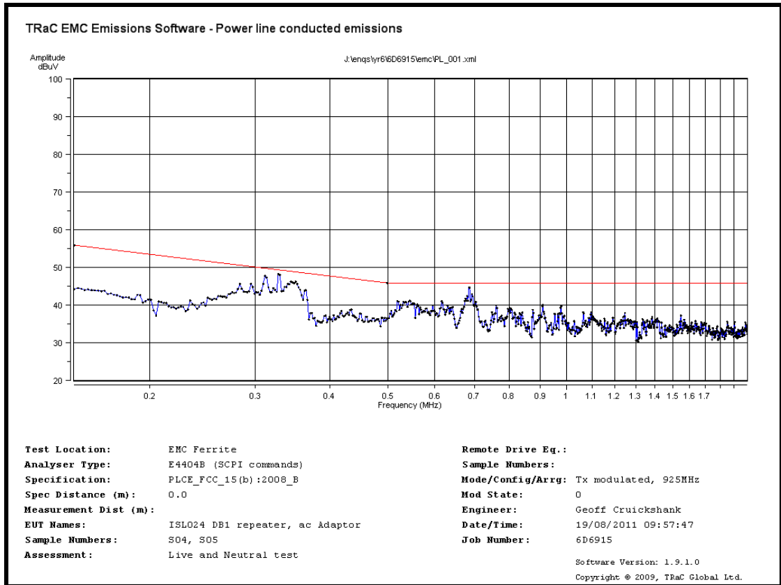
ac Power Line Conducted emissions 150kHz to 2MHz – Tx mode
