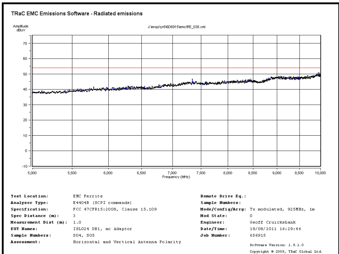
Radiated Spurious emissions 5 GHz to 10 GHz – Tx mode ac mains powered
