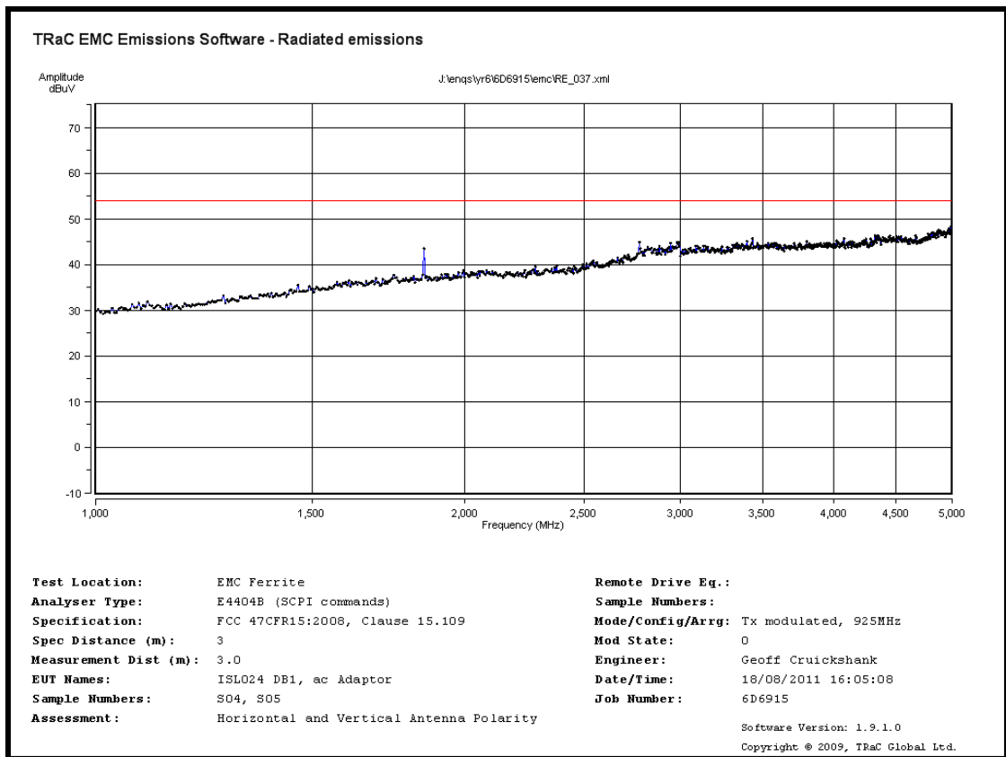
Radiated Spurious emissions 1 GHz to 5 GHz – Tx mode ac mains powered
