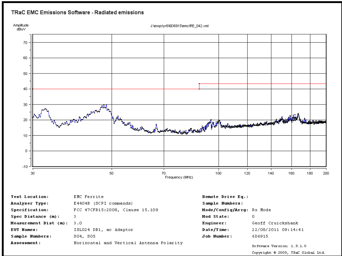
Radiated Spurious emissions 30 MHz to 200 MHz – Rx mode ac mains powered
