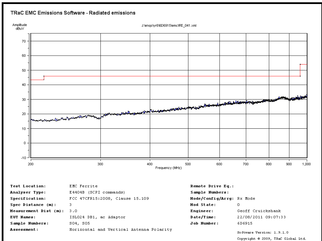
Radiated Spurious emissions 200 MHz to 1 GHz – Rx mode ac mains powered
