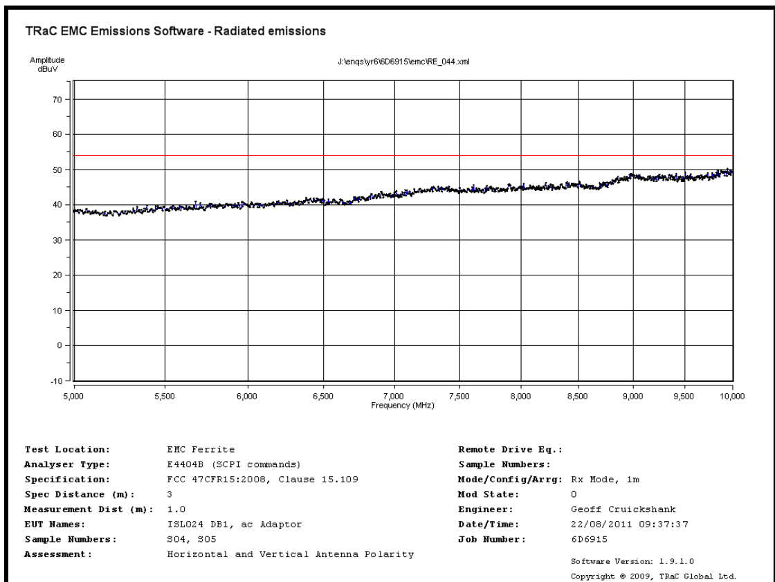
Radiated Spurious emissions 5 GHz to 10 GHz – Rx mode ac mains powered
