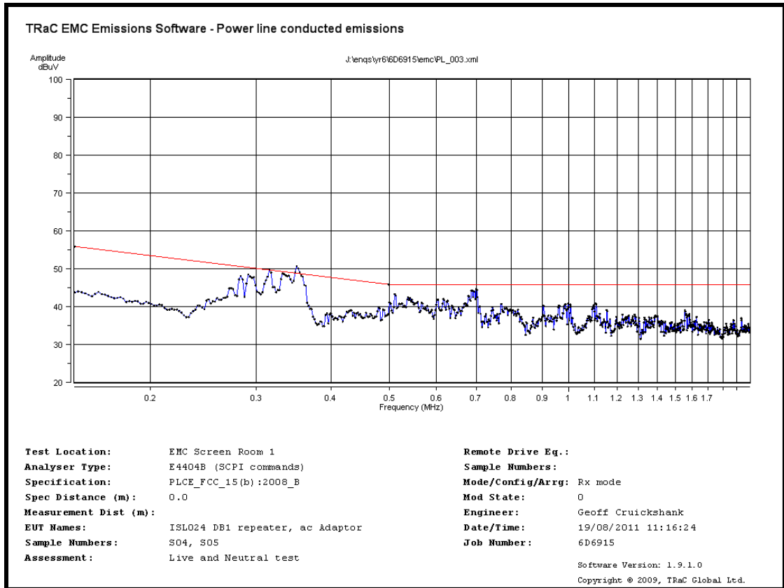
ac Power Line Conducted emissions 150kHz to 2MHz – Rx mode
