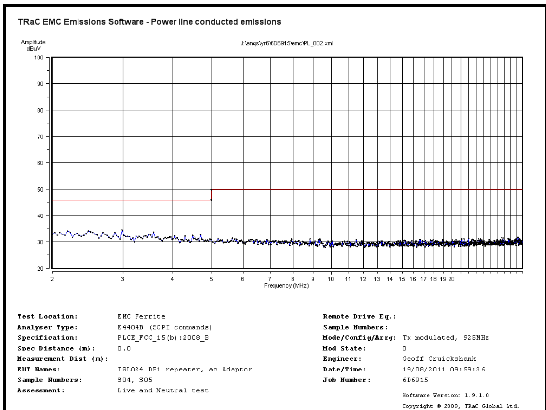
ac Power Line Conducted emissions 2MHz to 30MHz – Tx mode
