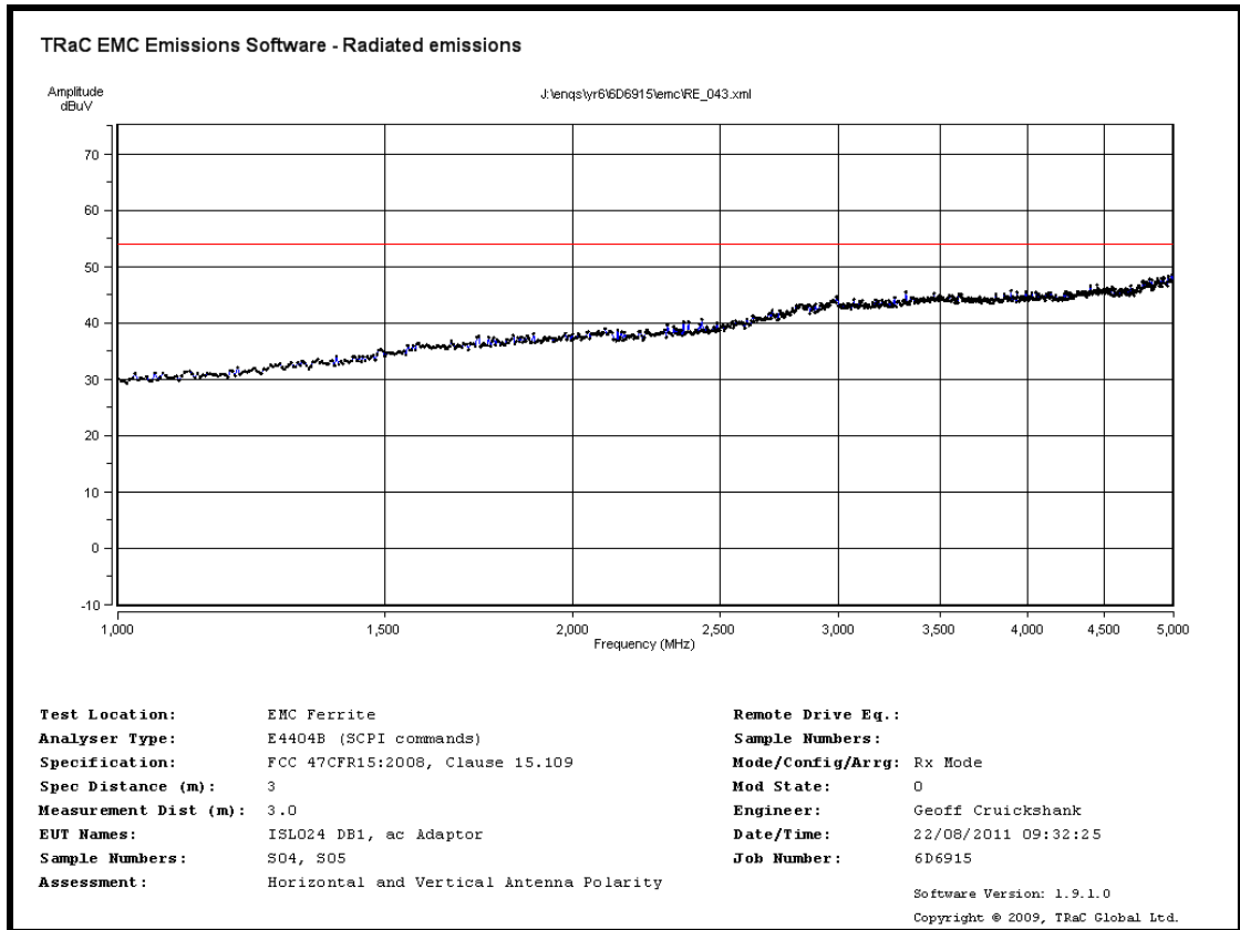
Radiated Spurious emissions 1 GHz to 5 GHz – Rx mode ac mains powered
