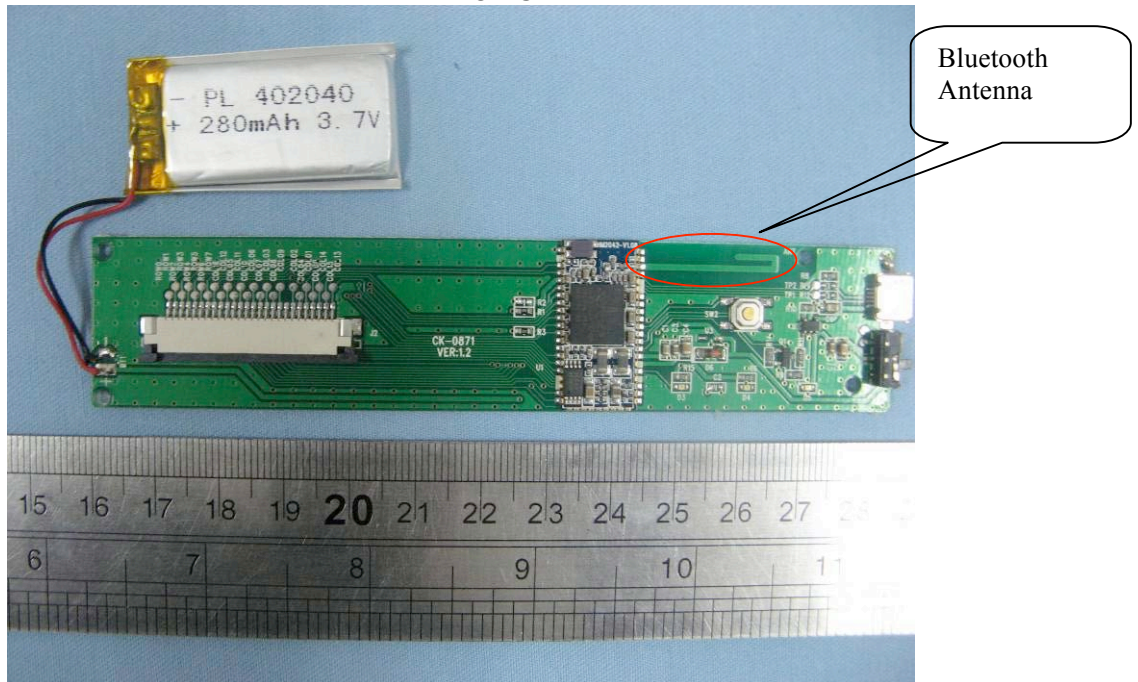
INTERNAL VIEW OF SAMPLE – 3
