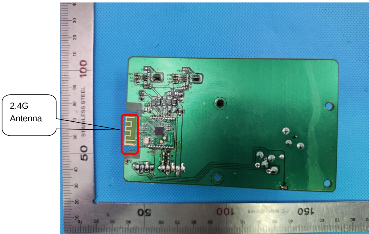
INTERNAL VIEW OF EUT (FIGURE 6)
