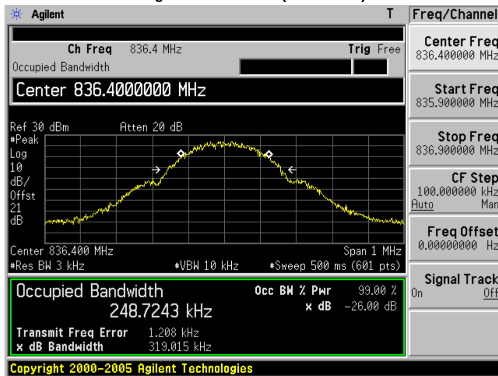
Figure Channel 189 (836.40MHz)
