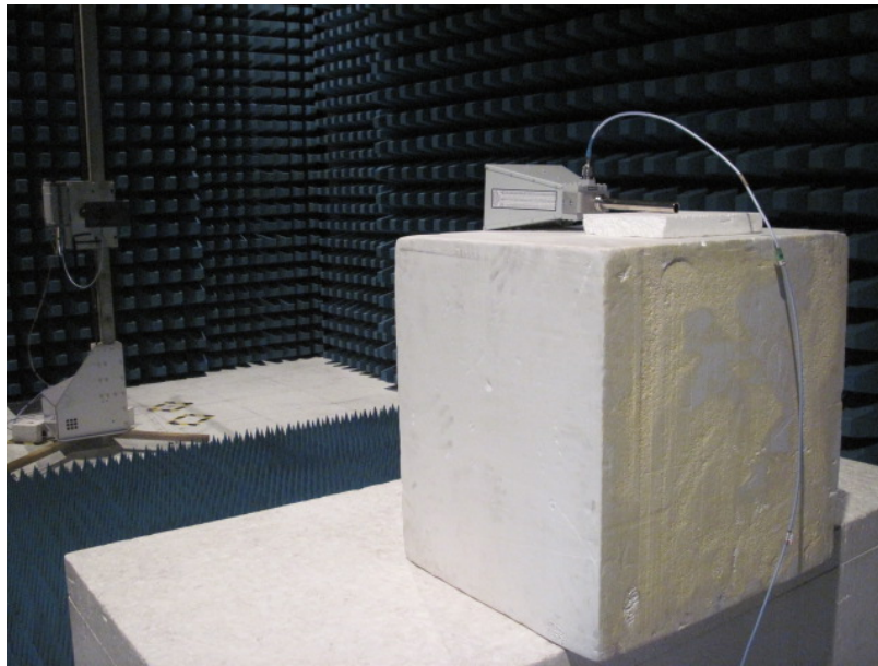
Description: Substitution Antenna for EIRP Test
