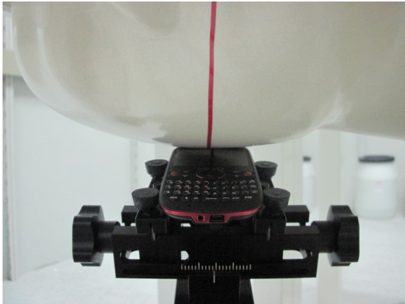
Right-Tilt 15°
