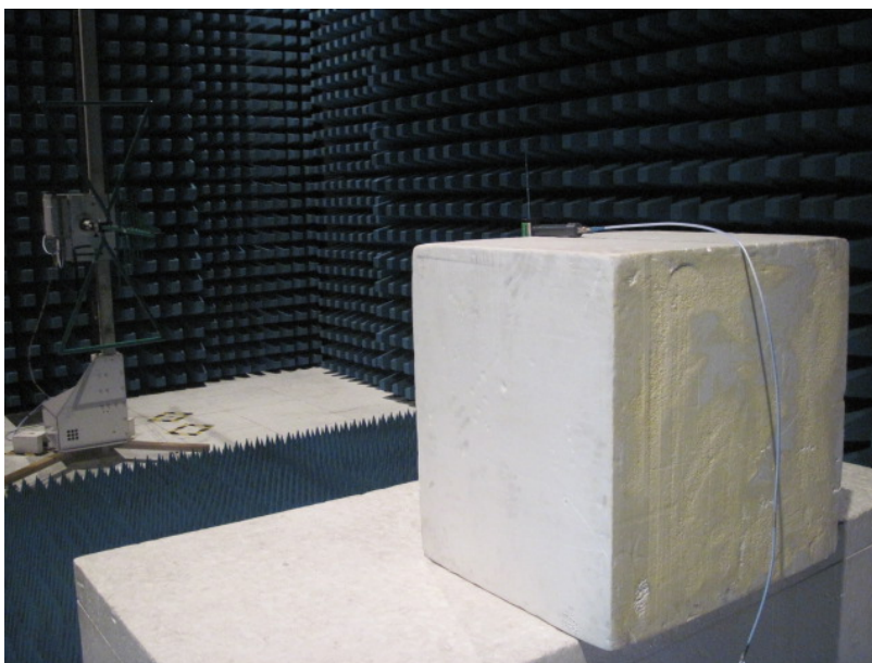
Description: EIRP Test Setup
