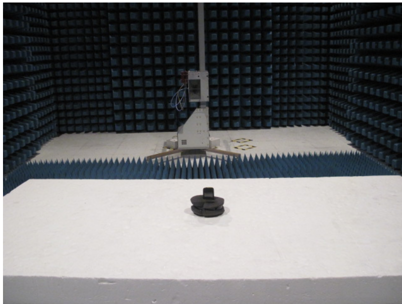
Description : Radiated Emission Test Setup for 1~18GHz
